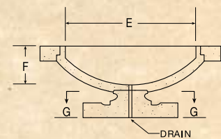
CUTAWAY
